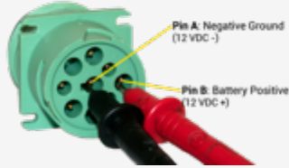
9-Pin Diagnostic Port
